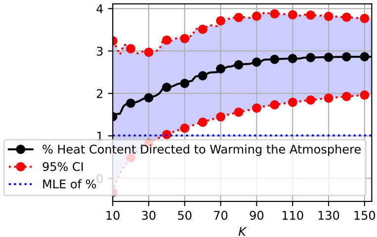
(b) % of Total Heat Content towards Surface Warming
