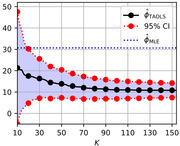
(a) TAOLS of \phi and 95% CI
